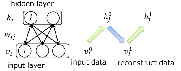
Fig. 4. The learning process of Restricted Boltzmann Machine.
