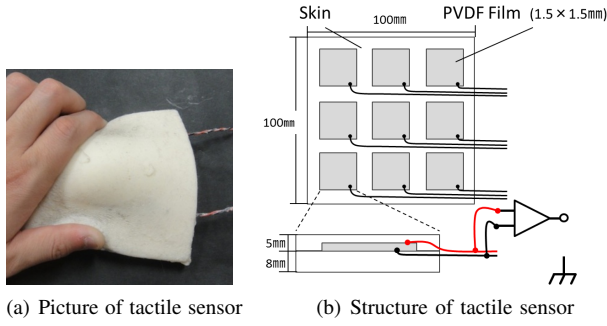
Fig. 5. The tactile sensor and its sample data. The sensor consists of urethane foam and PVDF films.
