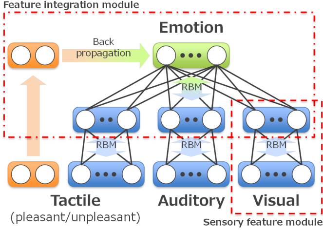
Fig. 3. A computational model of emotional differentiation based on tactile dominance in infancy. Each lower RBM network which is drawn by the blue connection (i.e., the region of enclosed broken lines) constitutes a Sensory feature module for the corresponding modality. The top layer of the RBM which is drawn by the green connection and emotional units which represent a rough emotion according to the superiority of emotional perception in sense of touch constitute a Feature integration module (i.e., the region of enclosed chain lines).
